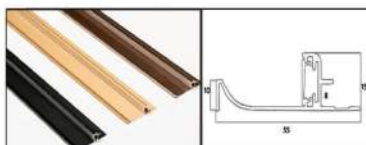
Model: 8513 Name: 8mm bottom luminous light strip skirting Color: matte black, matte gold, rose gold (from left to right)
