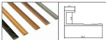
Model:5501 Name:5mm trimming line Color:Matte Black,Matte Gold,Matte Prestige Gold,Rose Gold,Matte Ink Grey(from left to right)
